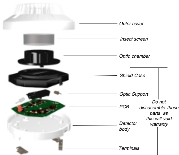
Figure 1:- 'Exploded' View of ST-P Detector Assembly
